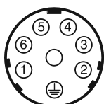
Brochage UV
