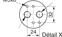
Type 2000U-4000U
