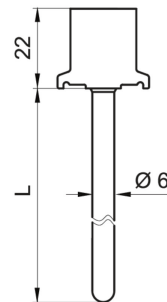
Tri-Clamp Ø 25 (BCID: C01)
