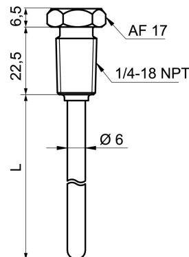
1/4-18 NPT (BCID: N01)
